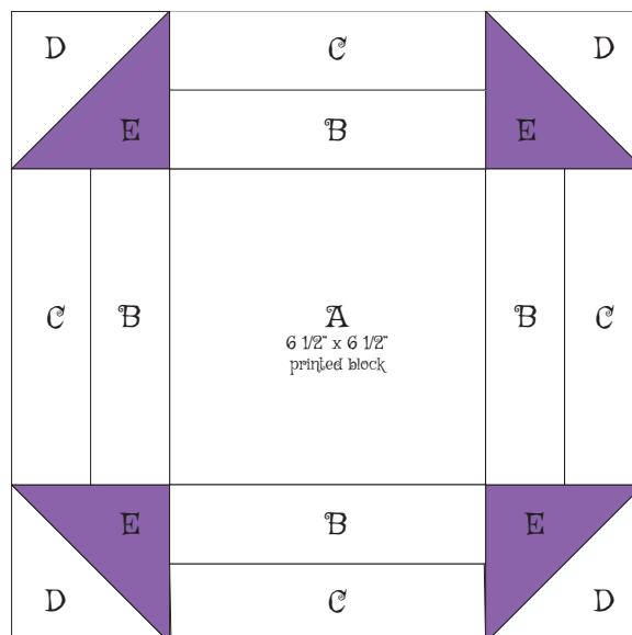
Block 2 Make 6
