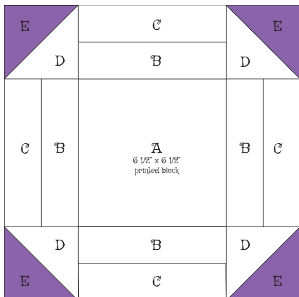
Block 1 Make 8
