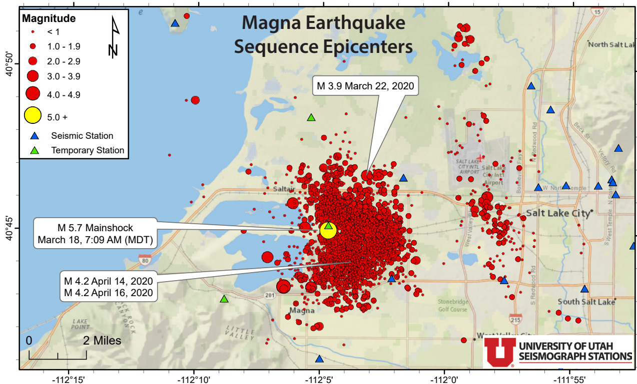
The UUSS has located 2,589 earthquakes as part of the Magna earthquake aftershock sequence from March 18, 2020, through March 18, 2022. The Magna earthquake shows that strong shaking from aftershocks can continue for months to years following the earthquake. Map courtesy of the University of Utah Seismograph Stations.
