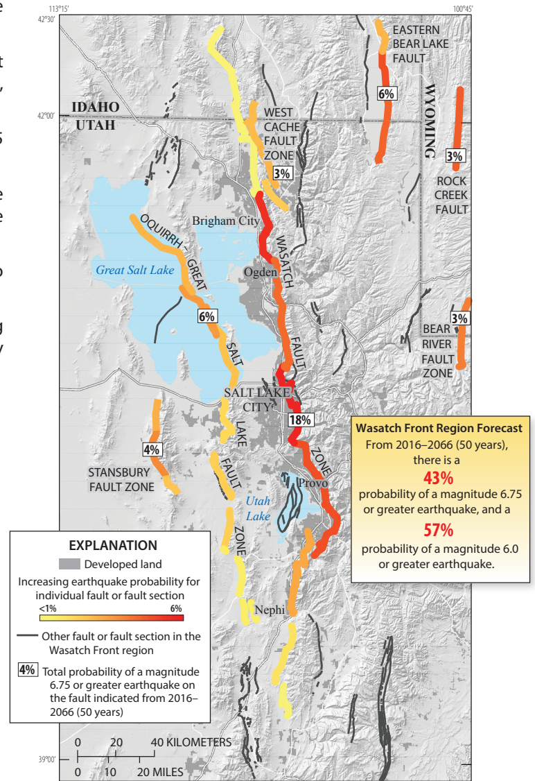
Magnitude 6.75 or greater earthquake probabilities may vary along faults (yellow to red fault colors). For example, the total probability for the entire Wasatch fault zone is 18 percent. Modified from the Working Group on Utah Earthquake Probabilities (2016).
