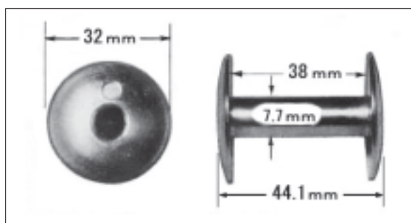
Large bobbin
