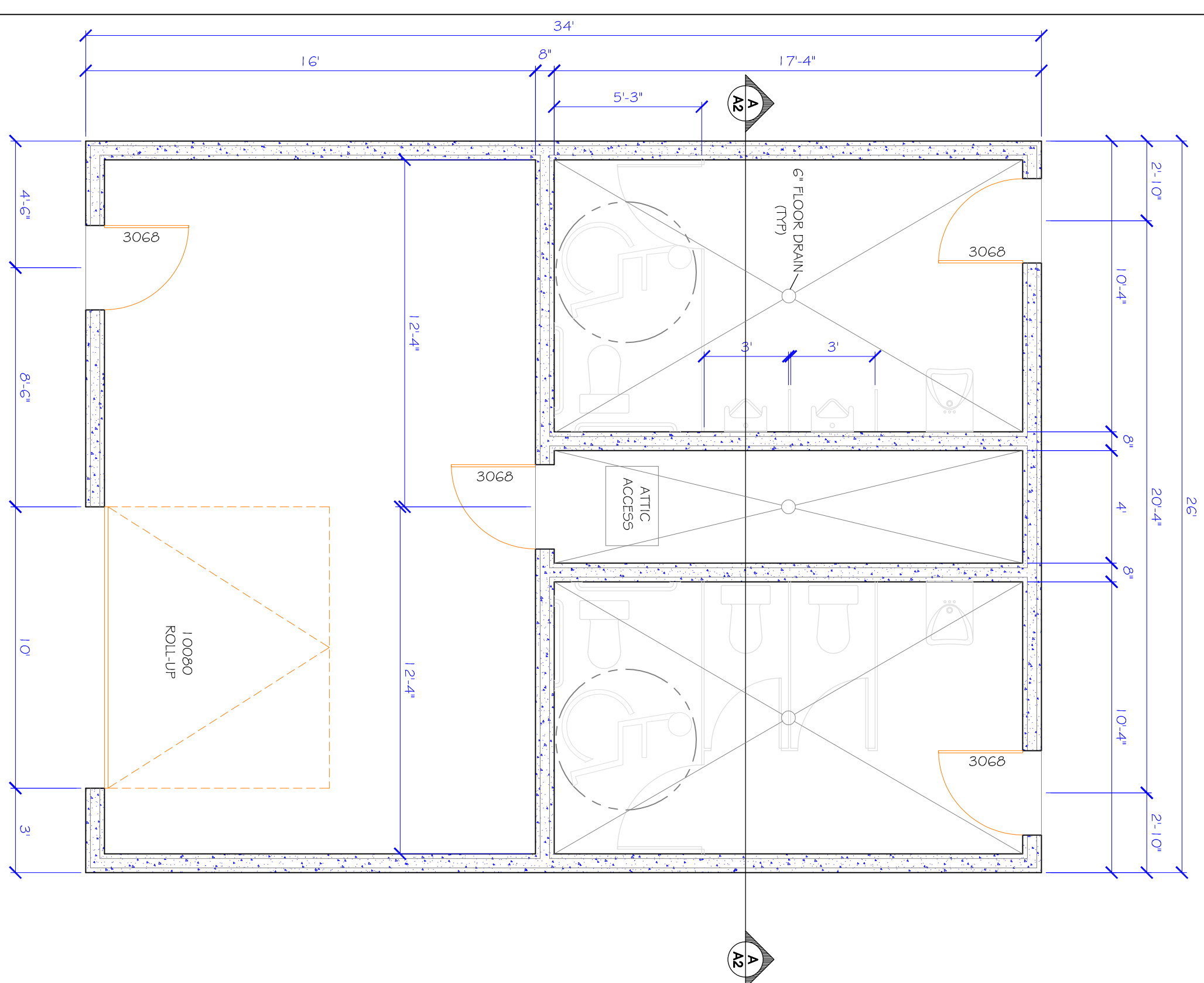
MAIN LEVEL FLOOR PLAN SCALE: 1/4" = 1'-0"
