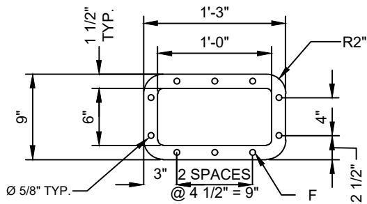
FLANGE DETAIL "D" ITEMS REMOVED FOR CLARITY. N.T.S.
