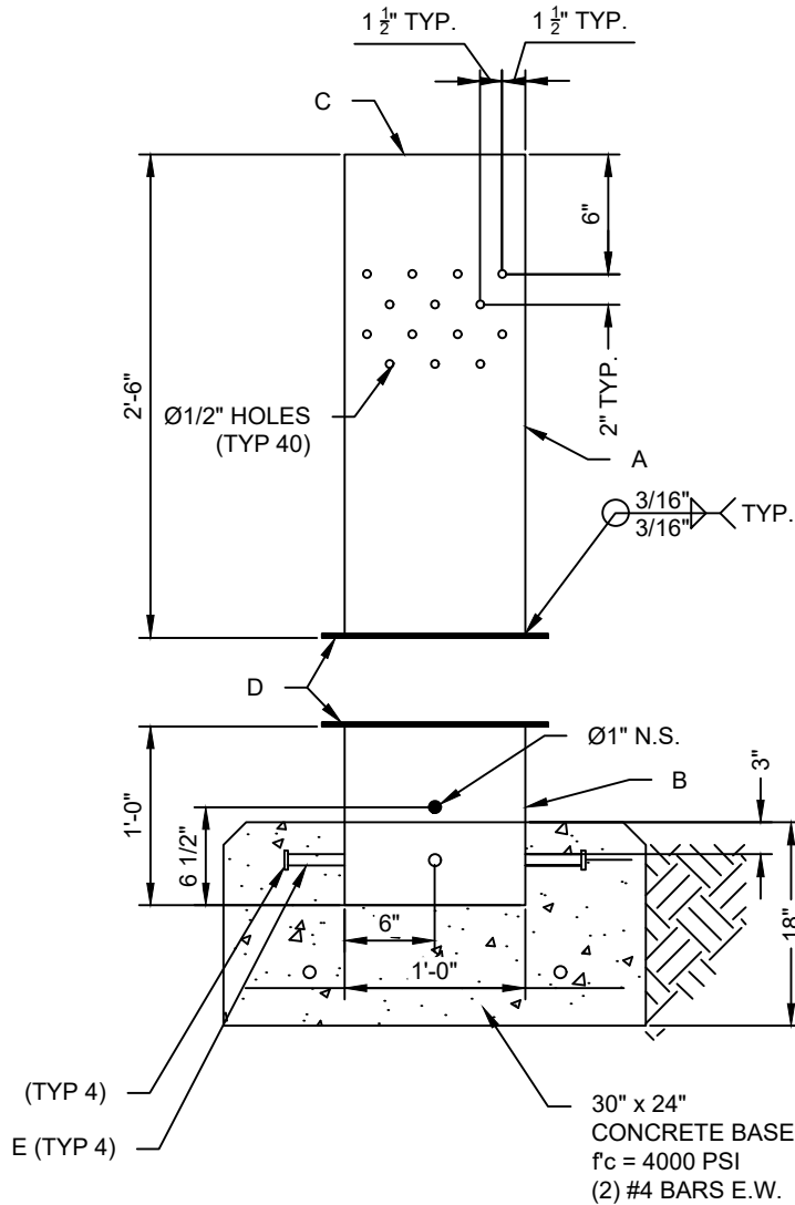
FLANGE DETAIL "D" ITEMS REMOVED FOR CLARITY. N.T.S.
