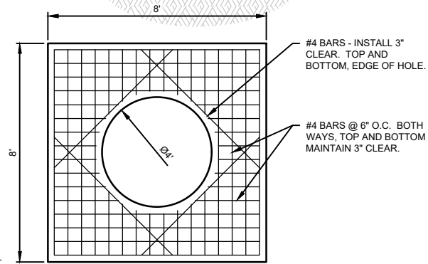
CONCRETE FOOTING
